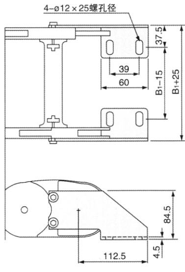
移动端/Moving Bracket
