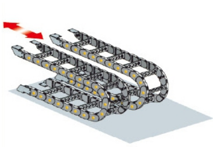
拖链平行运动 Chains positionted in parallel
