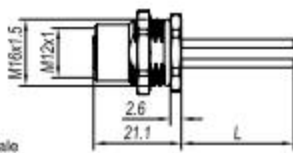
插孔尺寸图 Female
