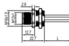
插针尺寸图 Male
