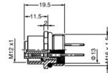
M12 插孔 Female
