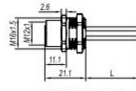
插孔尺寸图 Female
