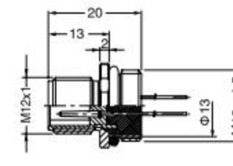
M12 插针 Male
