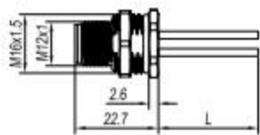
插针尺寸图 Male
