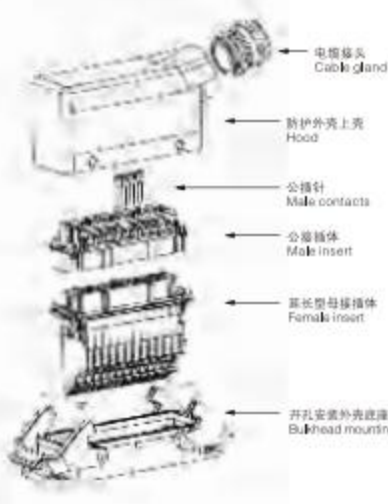
⑤ 穿孔安装，侧面进线形式 Through-panel connector and side entry type.
