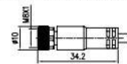
插孔 Female 直出 Straight 屏蔽 Shielded
