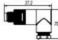
插针 Male 90°
