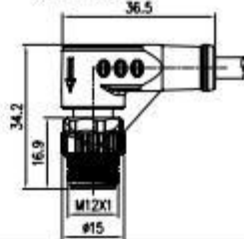
插针 Male 90°
