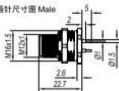
插针尺寸图 Male
