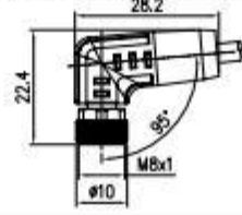
插孔 Female 90°
