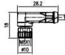
插孔 Female 90°
