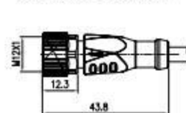
插孔 Female 直出 Straight
