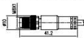
插针 Male 直出 Straight 屏蔽 Shielded
