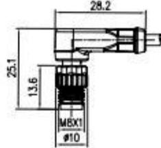
插针 Male 90° 屏蔽 Shielded
